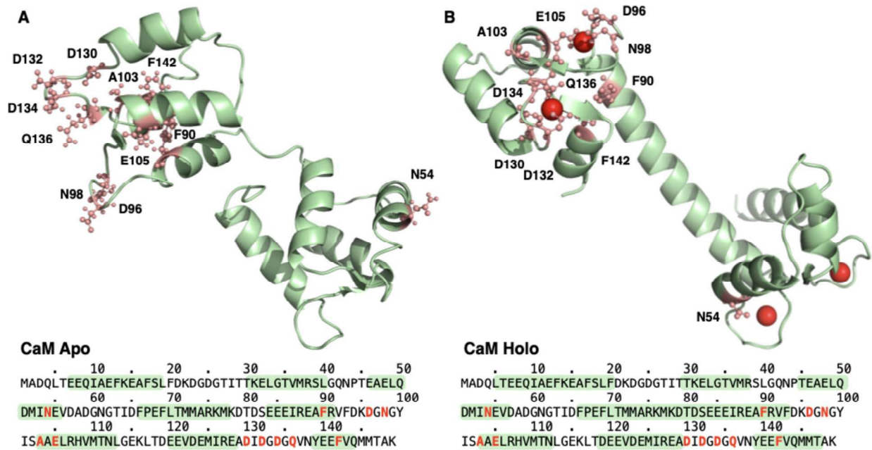
Fig. 1 Mapping of the 11 mutated sites corresponding to the 16 mutations from the CaM challenge dataset (shown in red) on the three-dimensional structures of calmodulin in its apo (A) and holo (B) forms. The structures for the apo and holo forms are derived from PDB entries 1DMO and 1CLL, respectively. In A, the variant aspar-
