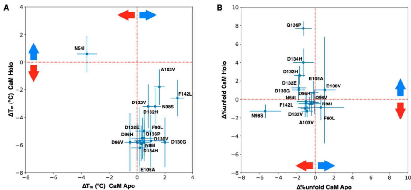
Fig. 2 Comparison of the changes in melting temperature ( A ) and %unfold ( B ) for the apo and holo forms of calmodulin. The change in melting temperature (ΔT m , panel A ) is calculated as ΔT m = T m mut - T m wt . B Shows the change in %unfold (Δ%unfold),
