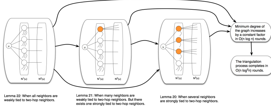
Figure 2.1: This figure illustrates the different cases and relations between lemmas used in the proof of Theorem 8. The shaded nodes in N_t^1(u) are strongly tied to N_t^2(u) . Others are weakly tied to N_t^2(u) .
