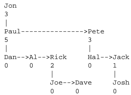
Figure 2: A sample Samizdat distribution system.
