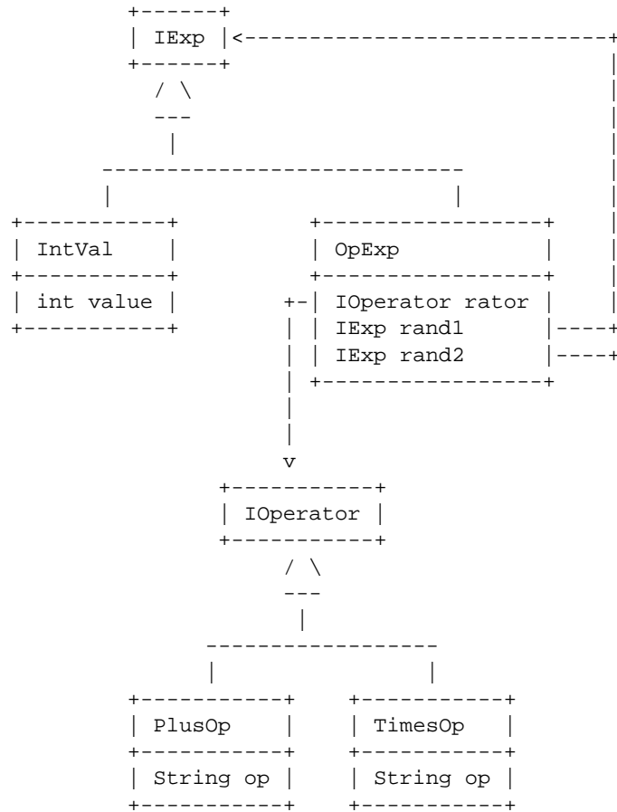
Figure 1: Representing arithmetic expressions.
