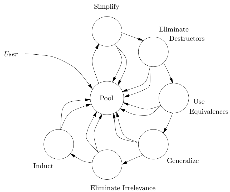
Figure 6.2: Organization of the Theorem Prover
